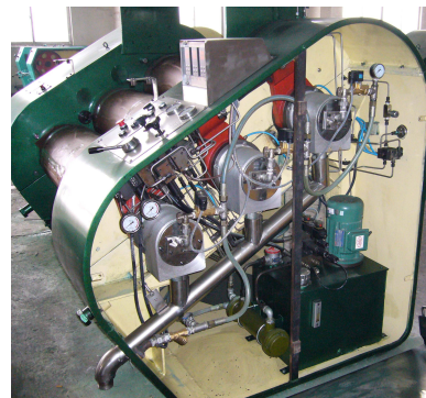
16" Hydraulic Model
